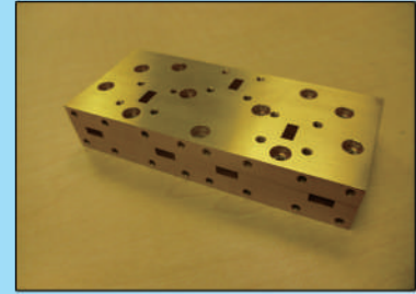
Waveguide Combiner
