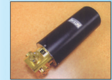
WR15 Electro-Mech Switch
