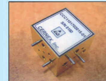
WR6 Crossguide Coupler
