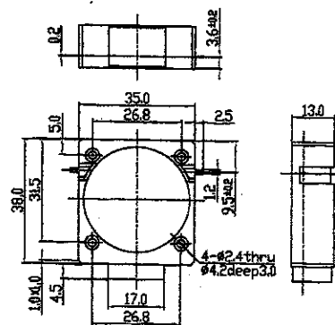
Package Drawing CB06
