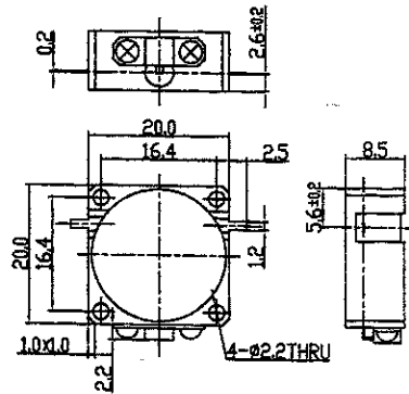
Package Drawing CB02
