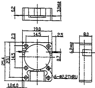
Package Drawing CB03
