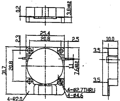
Package Drawing CB01
