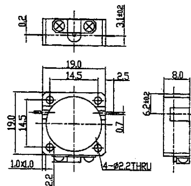
Package Drawing CB04
